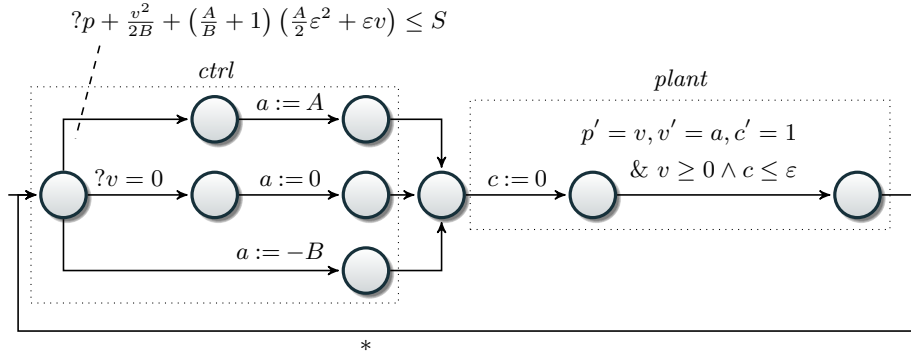
(a) State transition system
