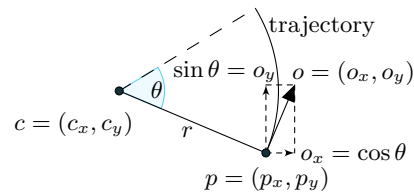
Fig. 12: State illustration of a car on a two-dimensional plane. The car has position p = (p_x, p_y) , orientation o = (o_x, o_y) , and drives on circular arcs of radius r and angle \theta around curve center points c = (c_x, c_y) .
