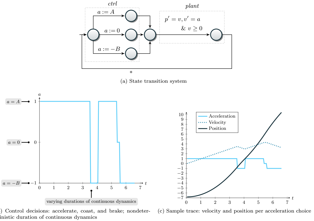
Fig. 4: A hybrid car controller (Example 2)
