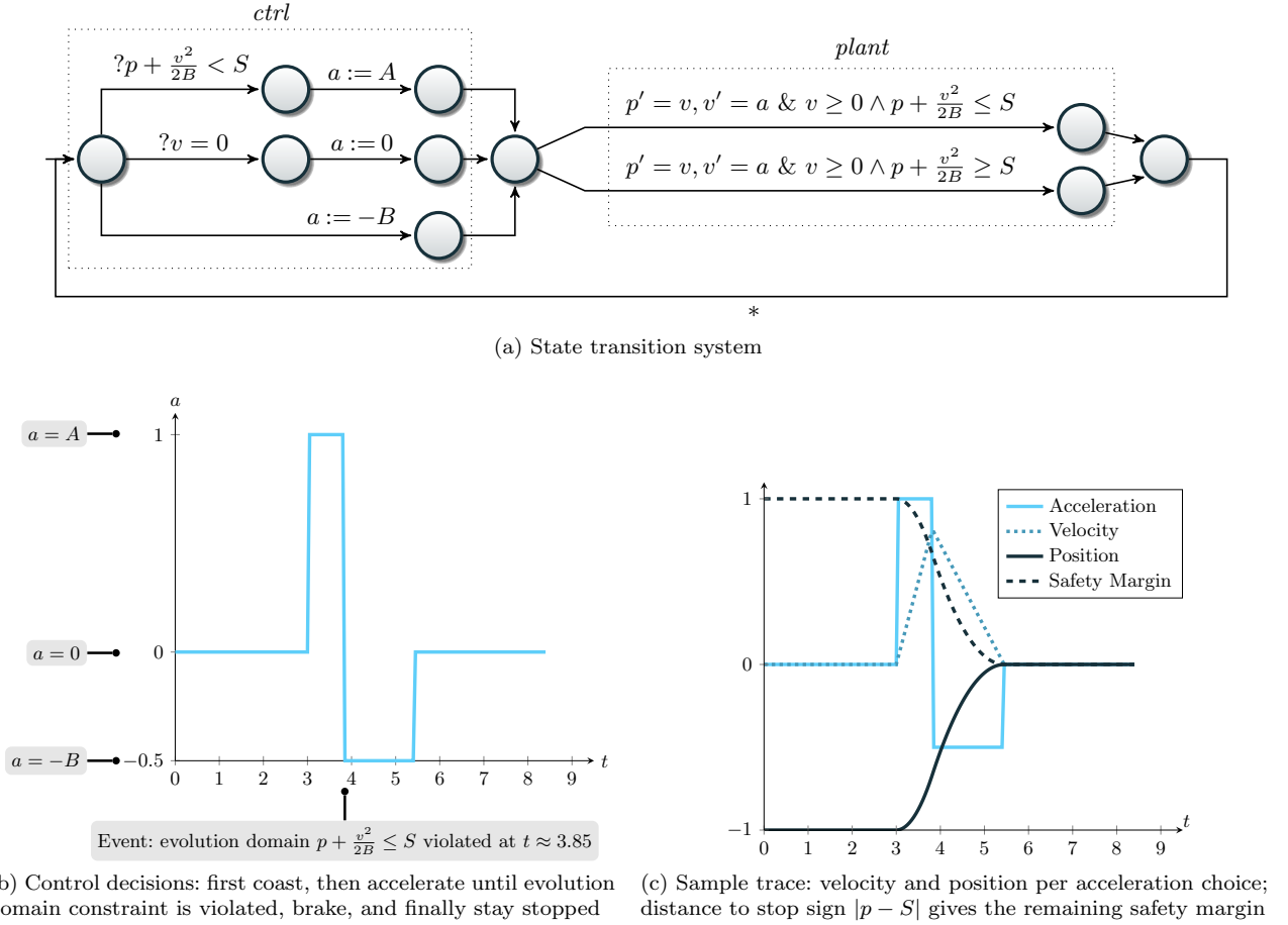
Fig. 5: Event-triggered stop sign controller (Example 3a)
