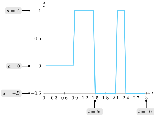
(b) Control decisions: despite nondeterministic loop duration c_i \leq \epsilon , the system was simulated with c = \epsilon
