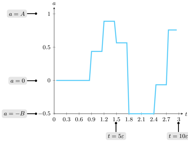
(b) Control decisions: nondeterministically chosen acceleration constrained with guard -B \leq a \leq A
