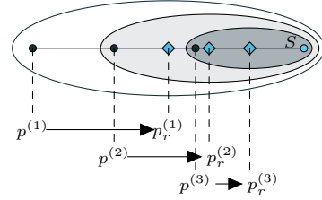
Fig. 10: Illustration of reference points set by the trajectory generator: point p^{(1)} moves towards reference point p_r^{(1)} until close enough, i.e. condition (72) holds at a point p^{(2)} , which is when the trajectory generator switches the reference point to p_r^{(2)} . Finally, at p^{(3)} the generator switches to p_r^{(3)} .
